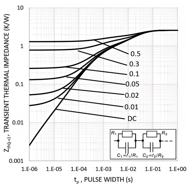
Fig. 18 FRD transient thermal impedance ( D=tp/T ) (TO-263)
