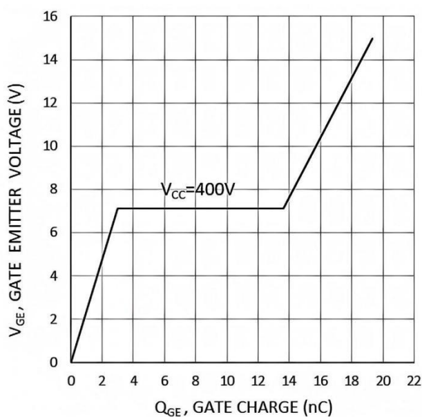
Fig. 16 Typical gate charge ( I_C=10A )
